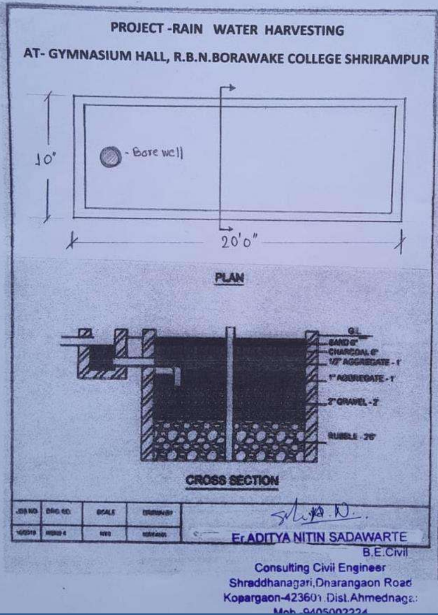
Rain Water harvesting project plan near Gymnasium Hall
